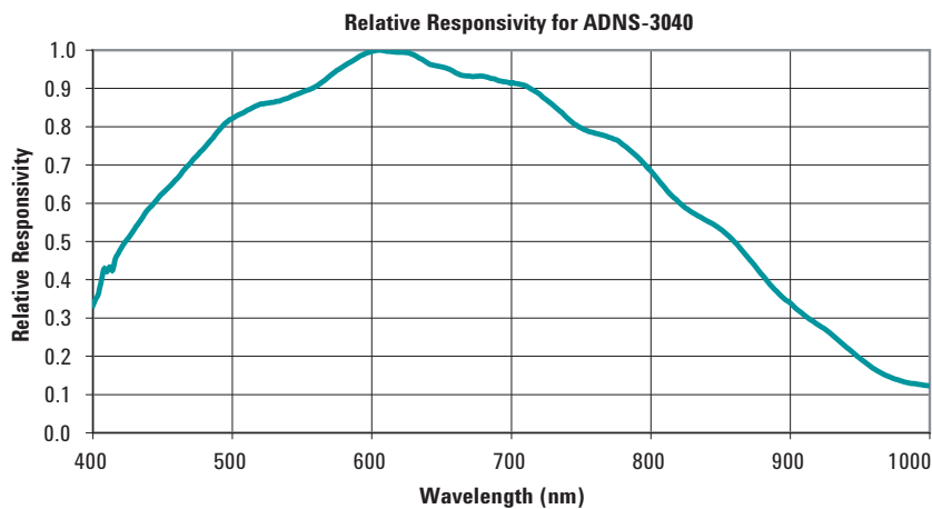
Figure 12. Relative Responsivity
